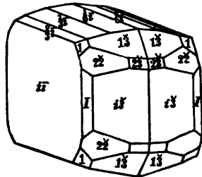
Greenland.
